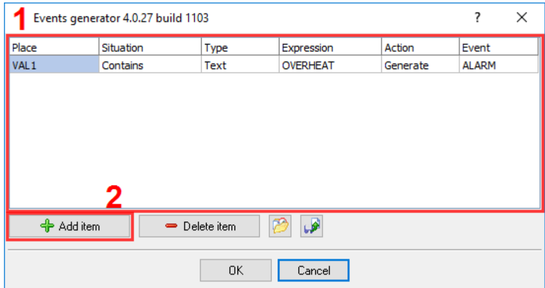
Fig.1 Filtering rules
