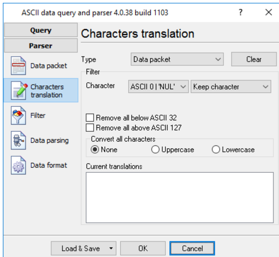
Fig.4 Character translation
