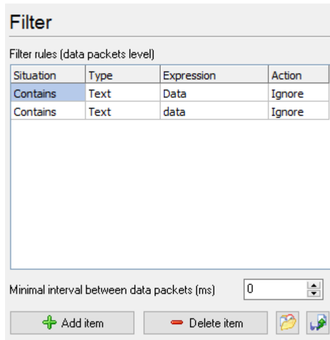
Fig.1 Filtering rules
