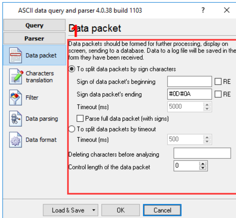
Fig.3. Data packets.
