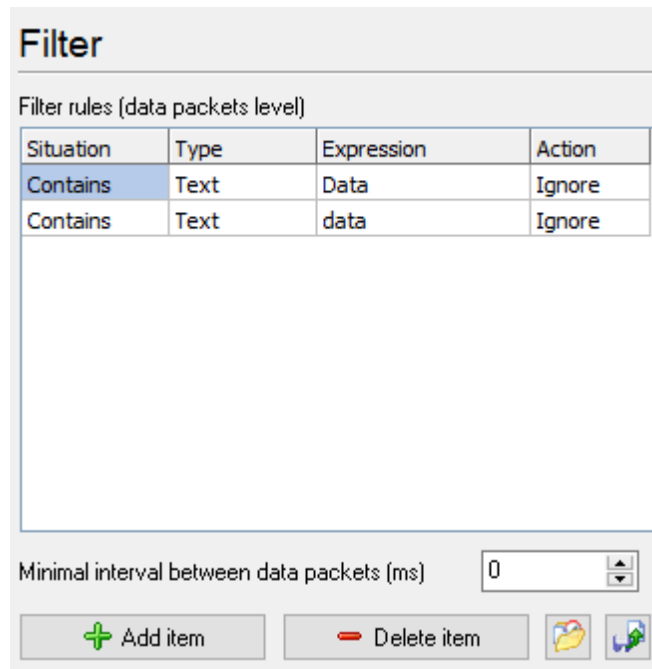
Fig.1 Filtering rules
