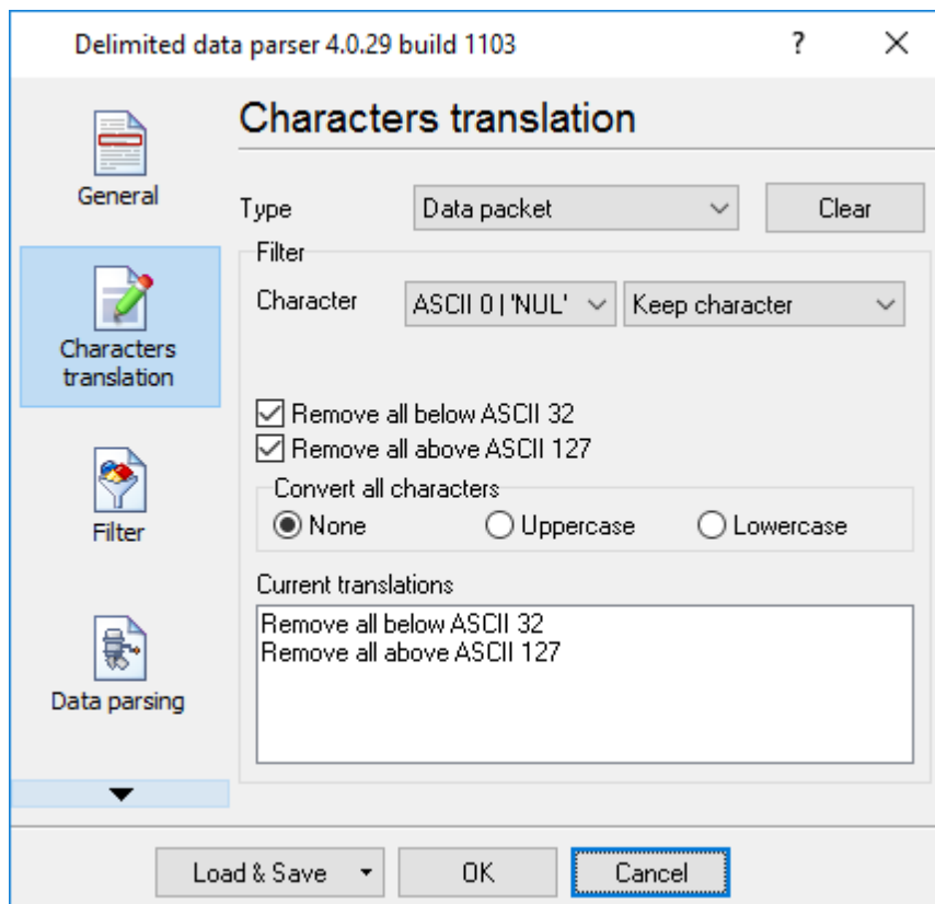
Fig.4 Character translation
