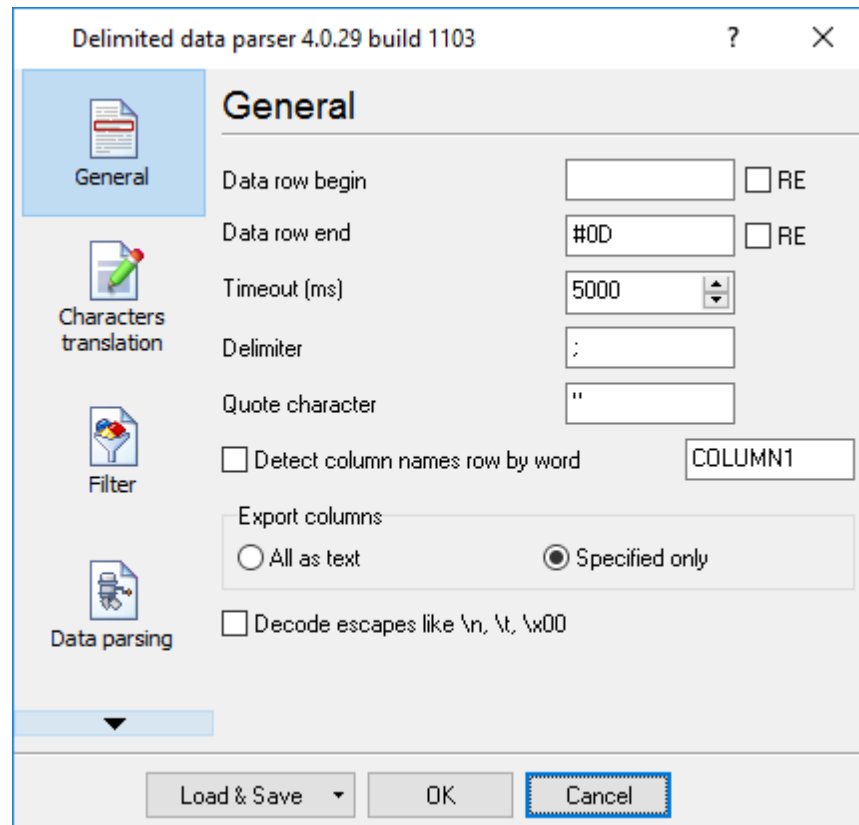
Fig.1. Data formatting.
