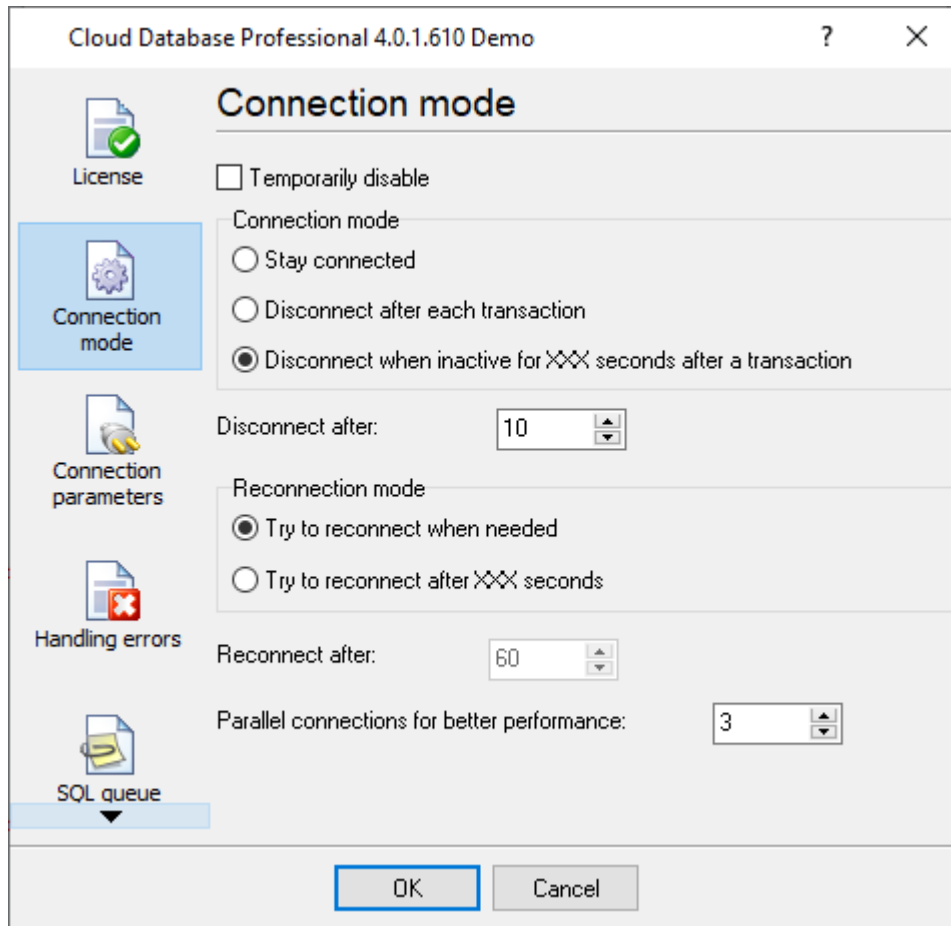
Fig. 1. Connection options
