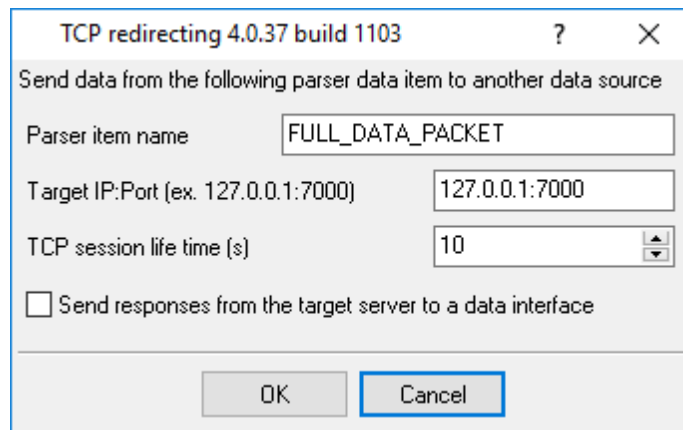
Figure 1: The settings window
