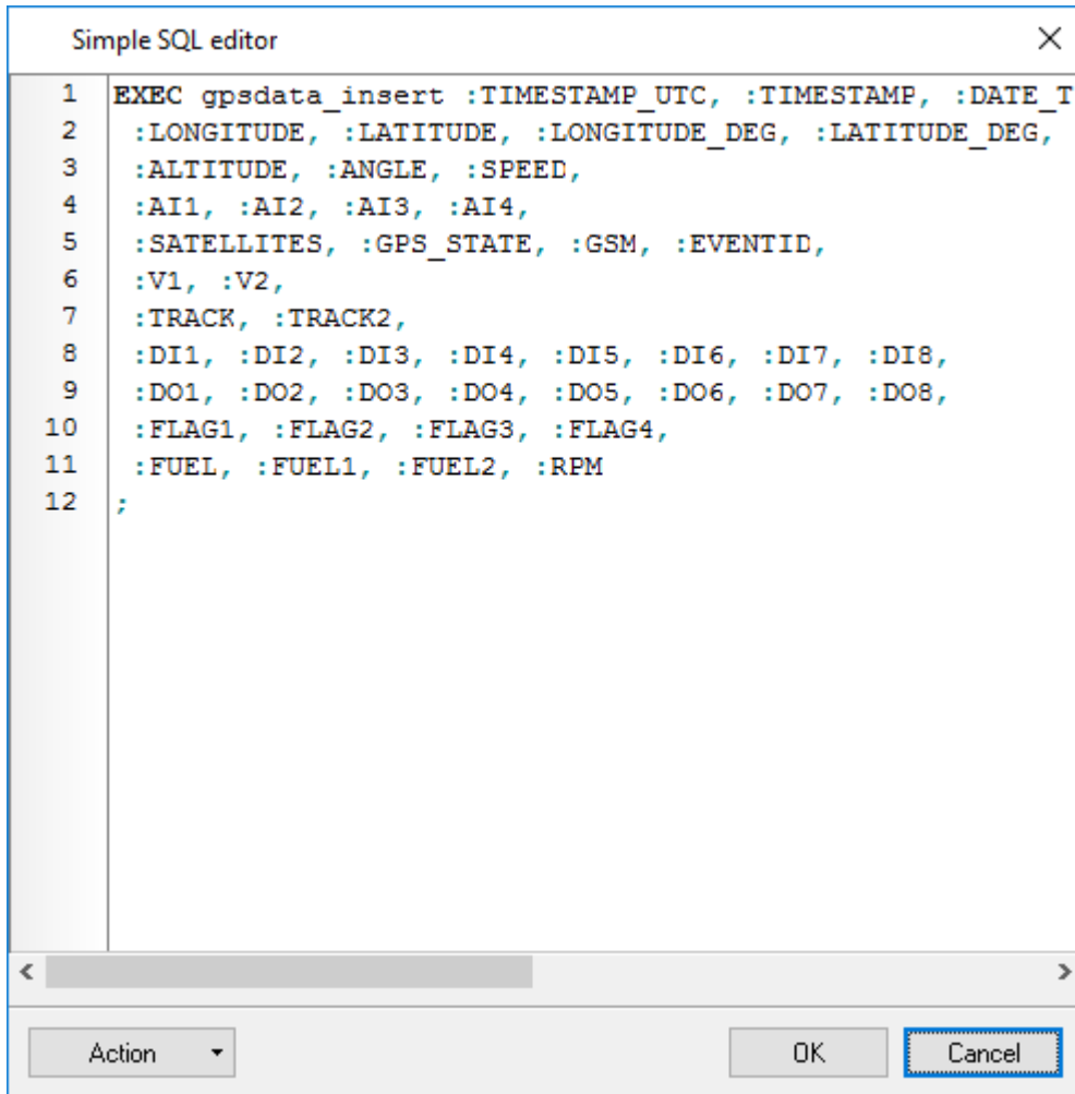
Fig. 6. SQL editor
